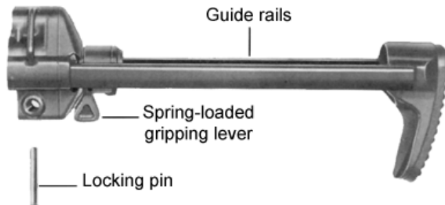
Fig. 18 Retractable buttstock
