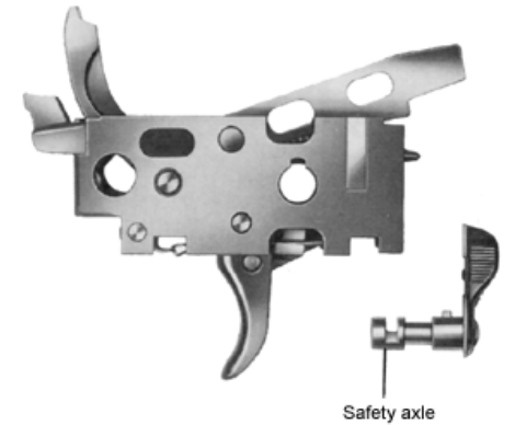
Fig. 16 Trigger mechanism and safety housing
